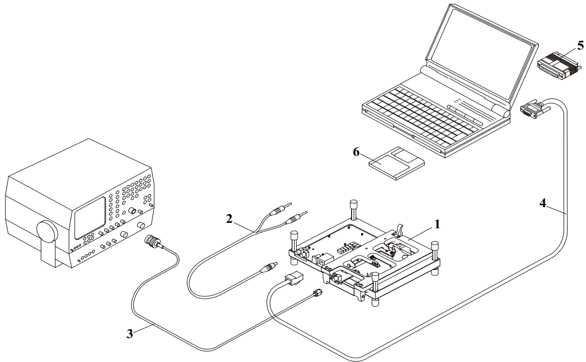
Figure 2: Module jig concept
