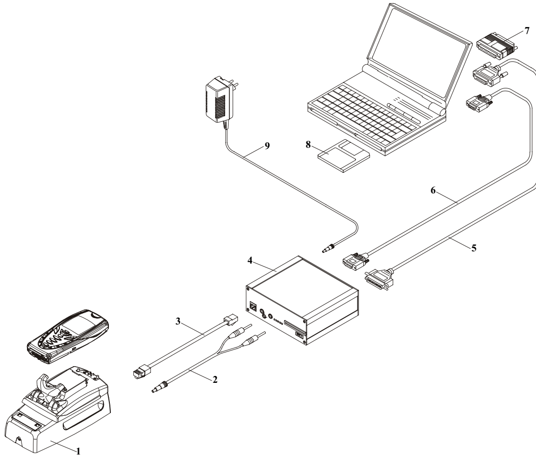
Figure 3: JBV-1 Flash concept
